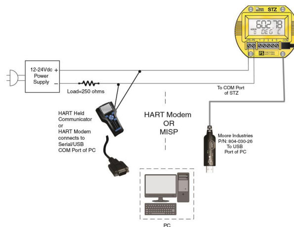
Figure 3: Schematic of the STZ’s interfaces
