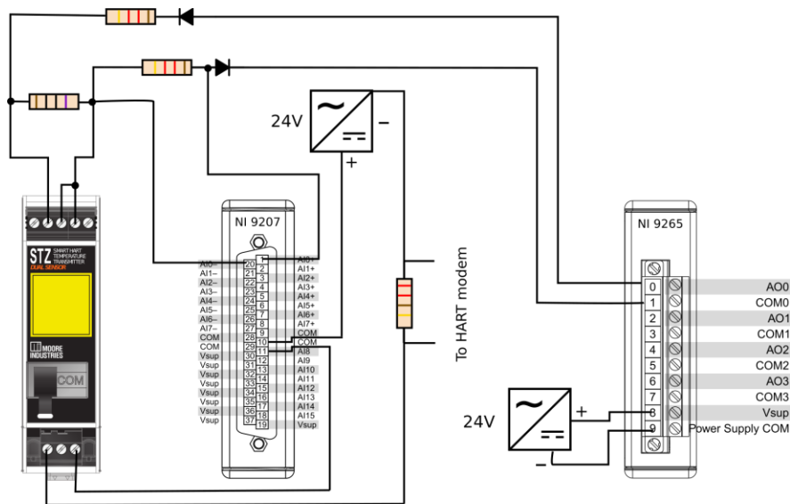
Figure 4: Schematic of the device-based testing apparatus
